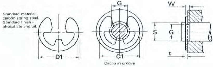
Circlip in groove
